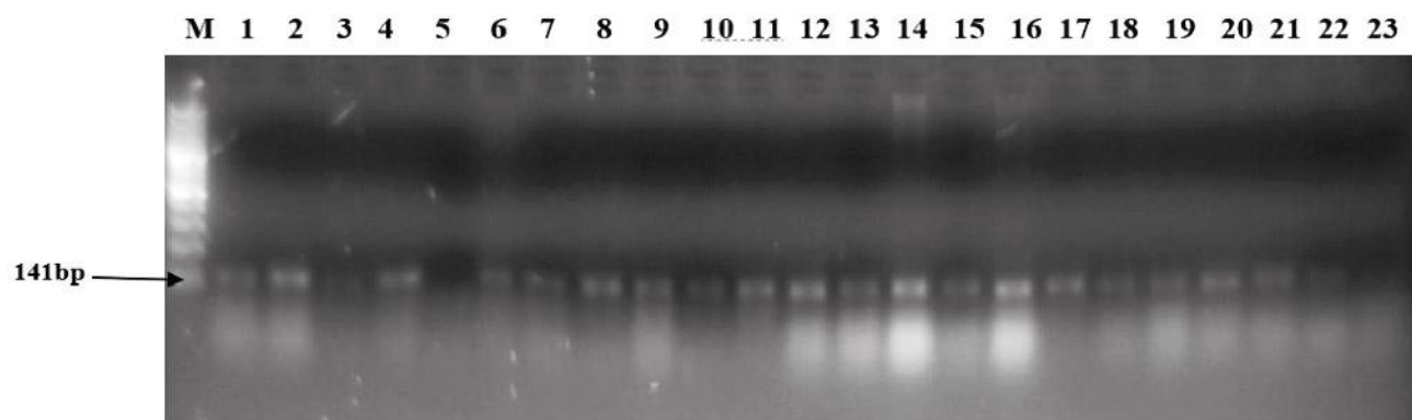
Fig. 1. DNA banding patterns of 23 rice accessions for identification of the BLB resistance gene Xa5
