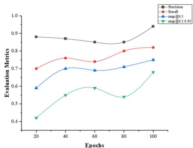
Fig. 11. Evaluation metrics at different training epochs.
