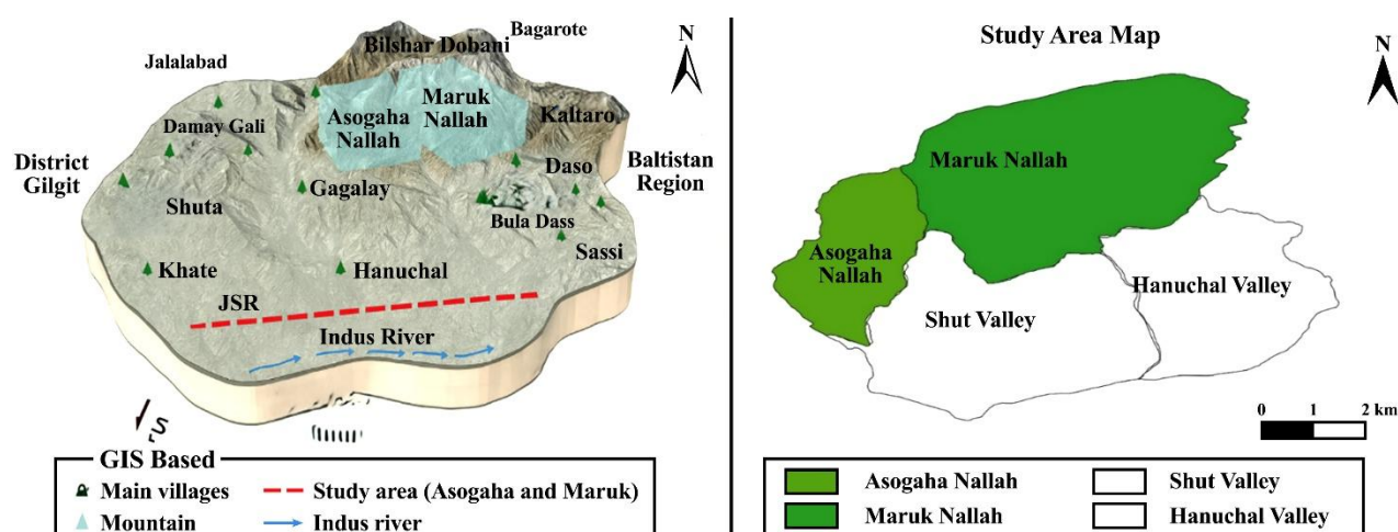
Fig. 1. Study Area Map of Maruk and Asogaha Nallah, Haramosh, District Gilgit.
