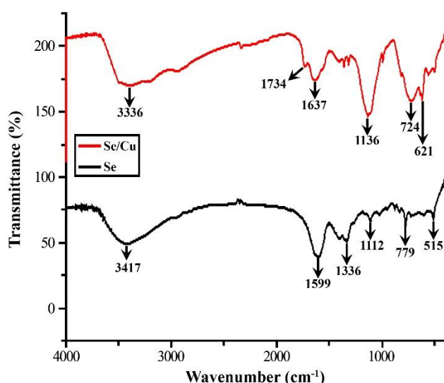
Fig. 2. FTIR of synthesized Se and Se/CuO NPs.
