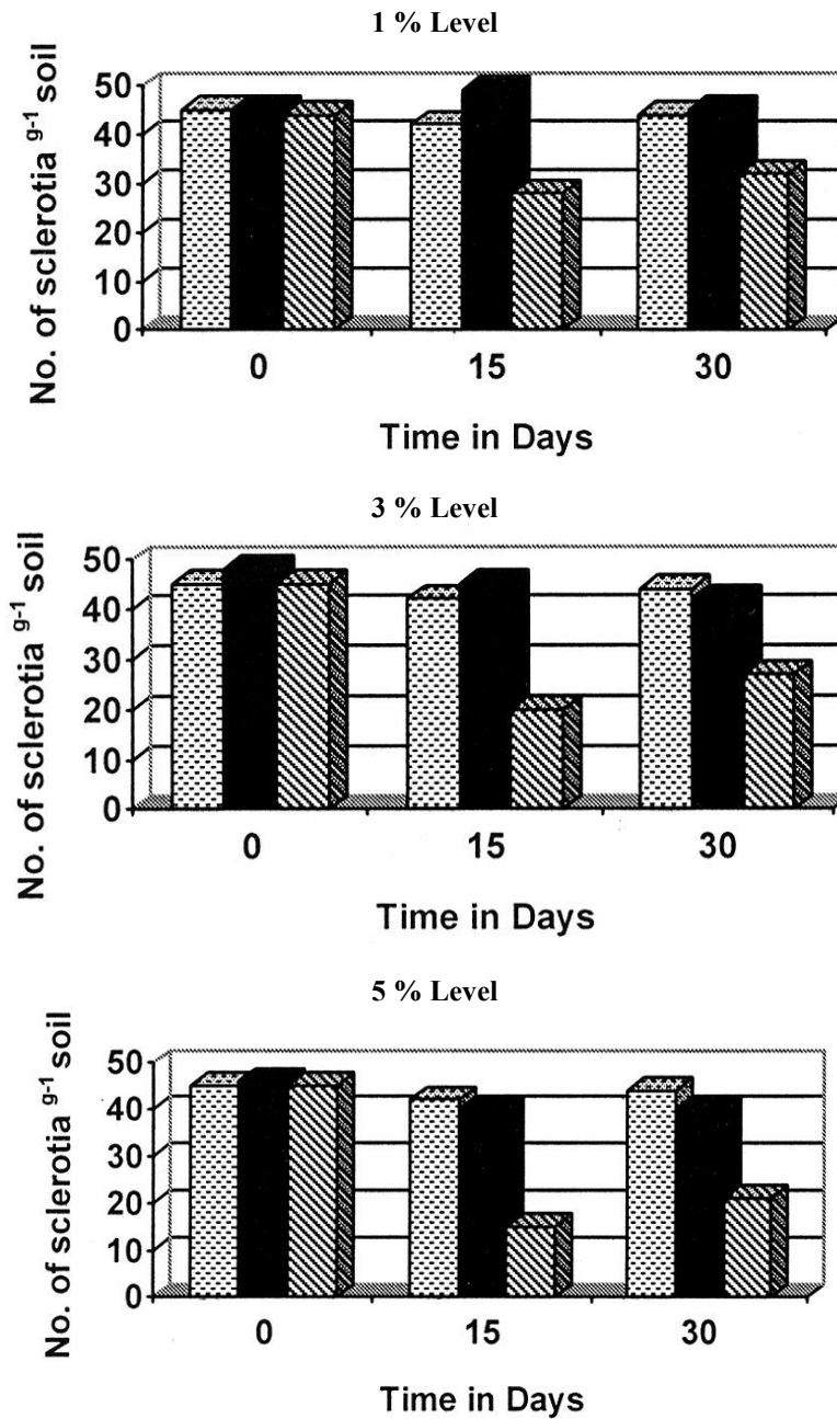
Fig. 1. Effect of poultry manure and sawdust used @ 1, 3 and 5% level on the reduction in number of sclerotia of Macrophomina phaseolina in soil at 40-50% MHC.
