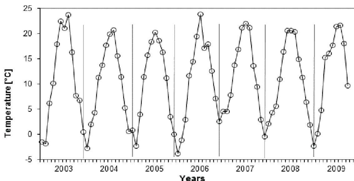
Fig. 3. Monthly average temperature per month for the Bratislava Koliba Meteorological Station during period of 2003-2009 years.
