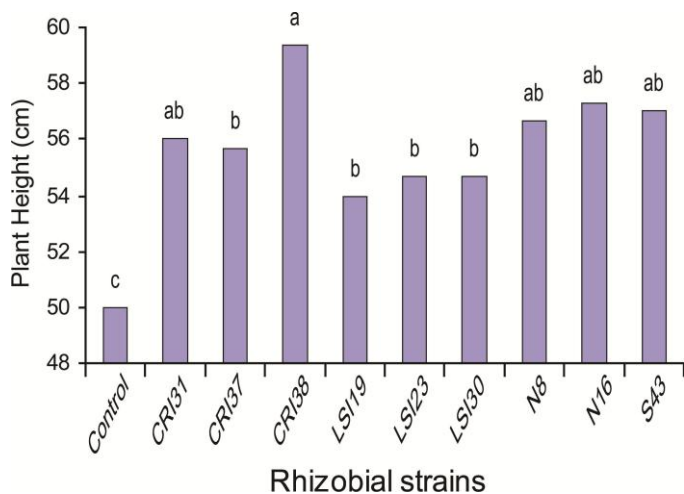
Fig. 1. Effect of inoculation with different species of rhizobia on plant height of wheat plants grown in pots.
