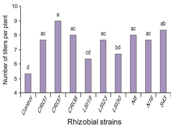
Fig. 2. Effect of inoculation with different species of rhizobia on number of tillers per plant of wheat plants grown in pots.
