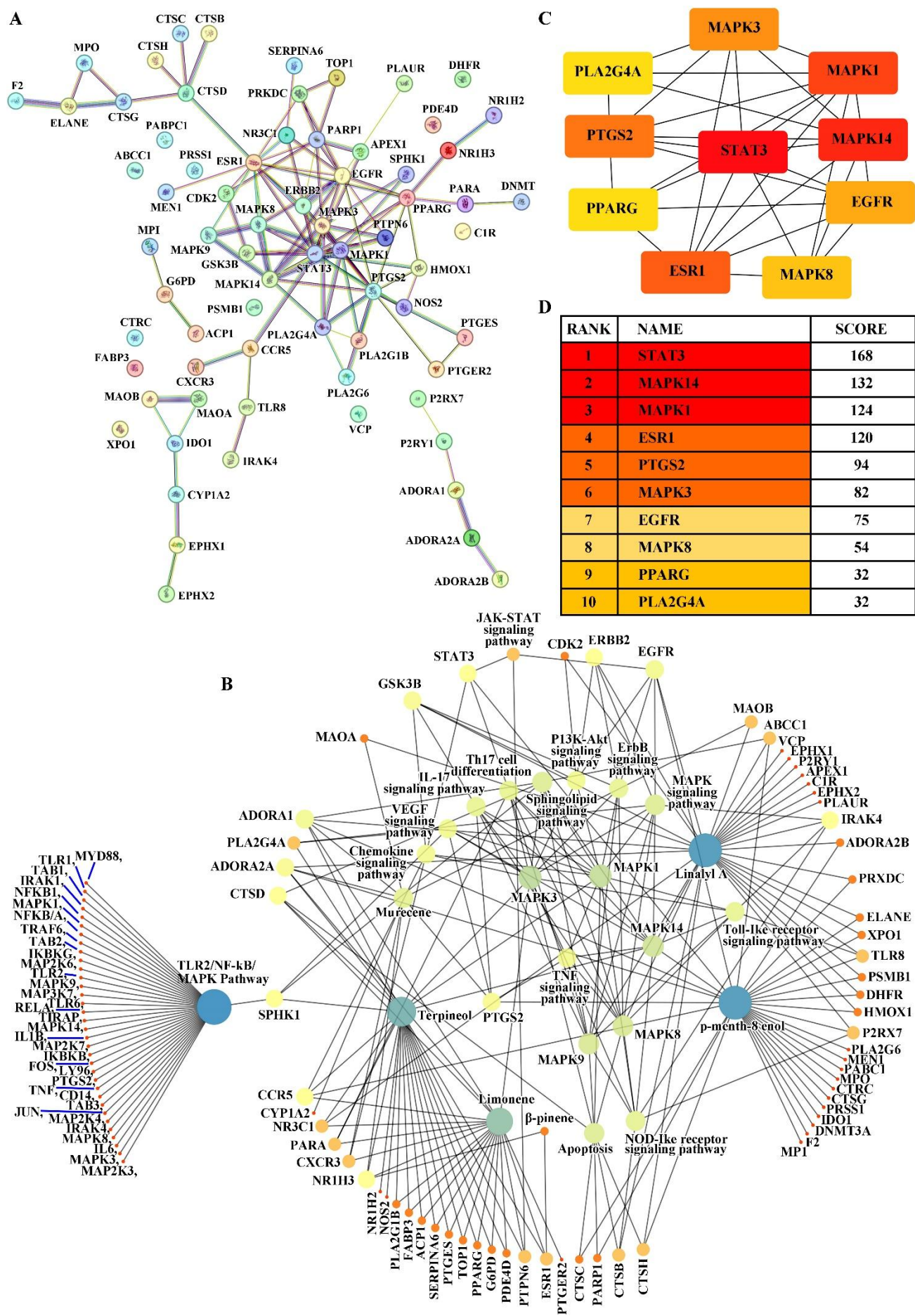
Fig. 4. A detailed overview of network analysis using PPI network (A), cytoscape merged networks (B), and hub genes (C).
