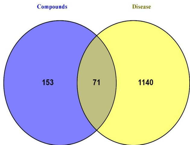
Fig. 3. Venn diagram showing common genes.
