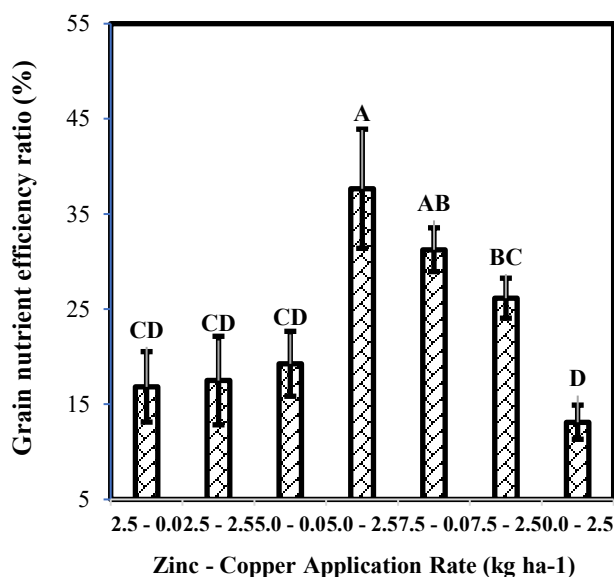
Fig. 1. Grain-to-nutrient efficiency ratio of wheat in relation to single and integrated application of zinc and copper at different rates. Error bars represent ± standard error of the mean based on three replications. CV (%) = 18.73; HSD (0.05) = 3.093.
