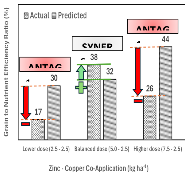
Fig. 2. Nature of zinc and copper interaction in response to their co-application at lower, balance and higher application rates in wheat.
