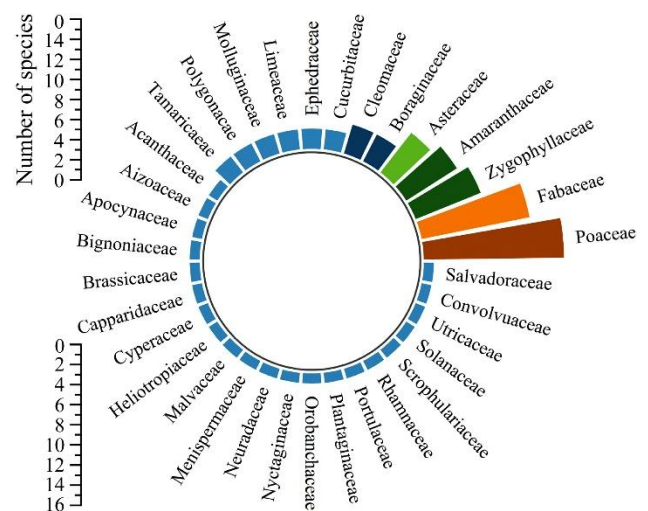
Fig. 2. Plant families and species richness of Takkar Wildlife Sanctuary Khairpur District.
