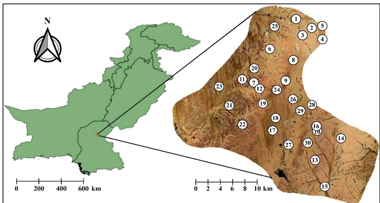
Fig. 1. Distribution of the sampling location within the boundaries of study area (Takkar Wildlife Sanctuary) and the location of study area in Sindh Province of Pakistan.
