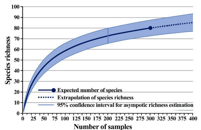
Fig. 3. Species accumulation curves using extrapolation (dashed curves) with 95 confidence interval for asymptotic species richness estimation in given samples from Takkar Wildlife Sanctuary (Colwell, 2013). Y-axis shows the number of species and X-axis shows the number of samples.
