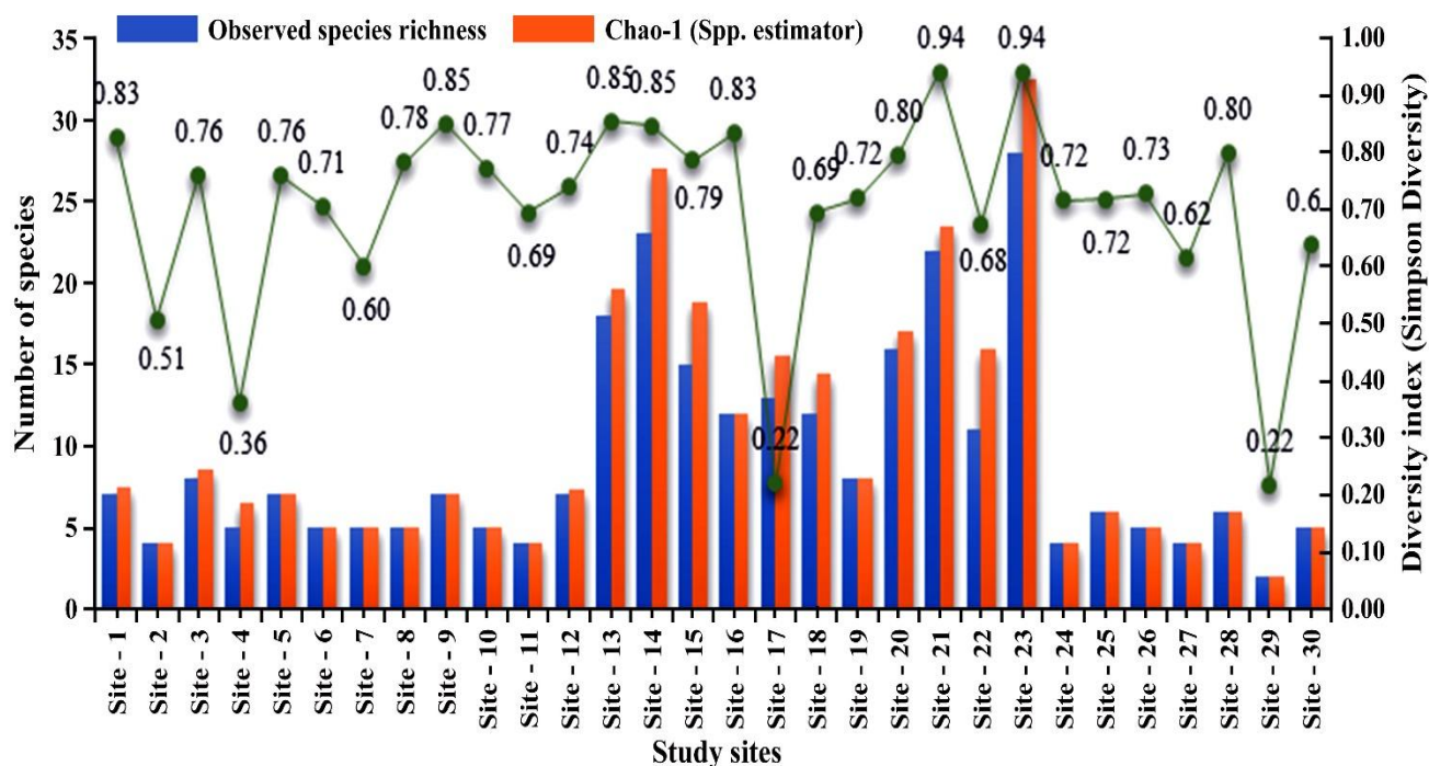
Fig. 4. Species richness and diversity of species at various study sites at Takkar Wildlife Sanctuary.
