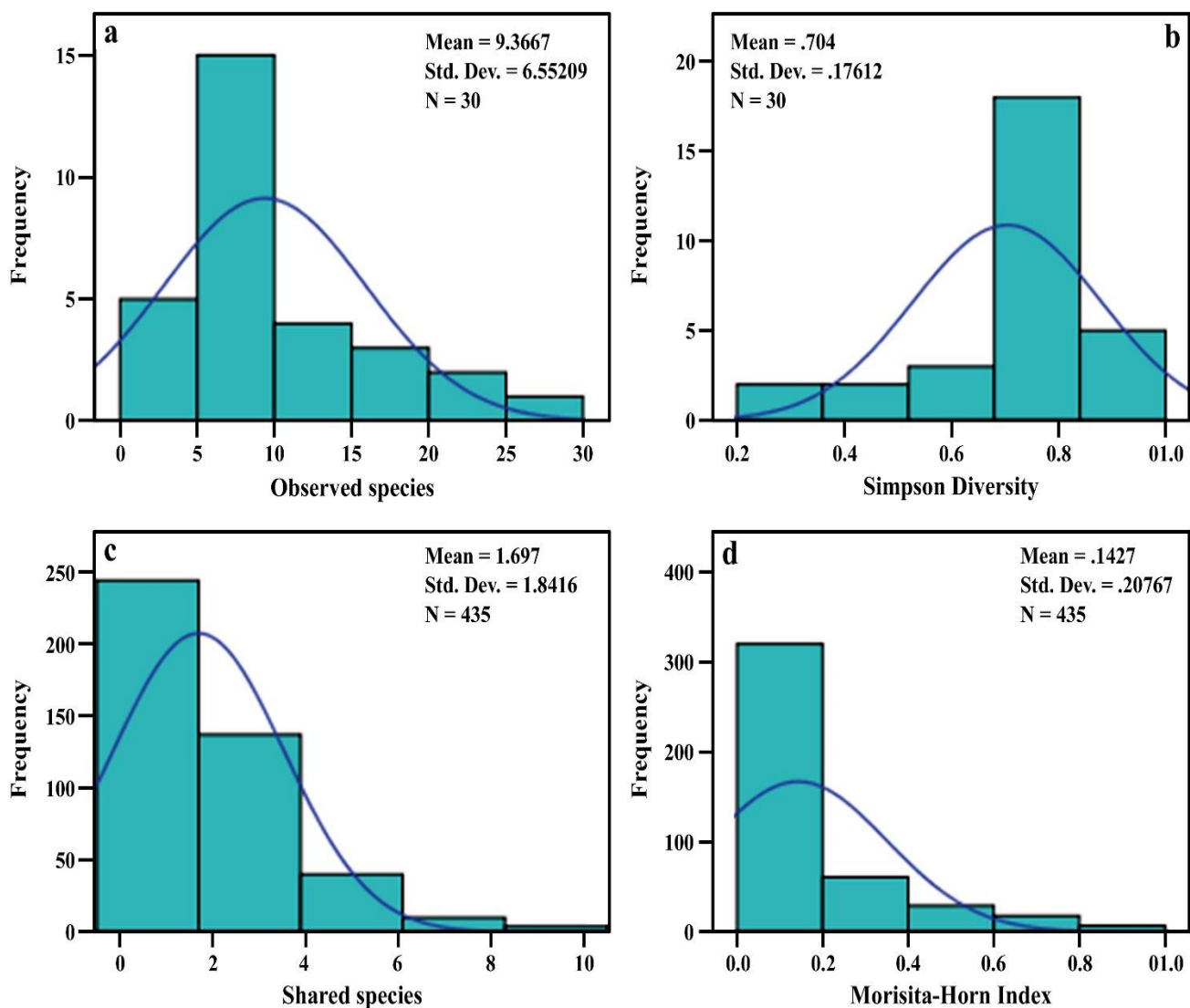
Fig. 5. Frequency distribution of community parameters: a, Observed species; b, Simpsons diversity; c, Shared species; d, Morisita-Horn index.
