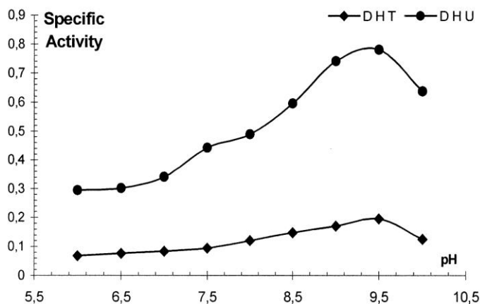
Fig. 4. The effect of pH on DHPase activity.
