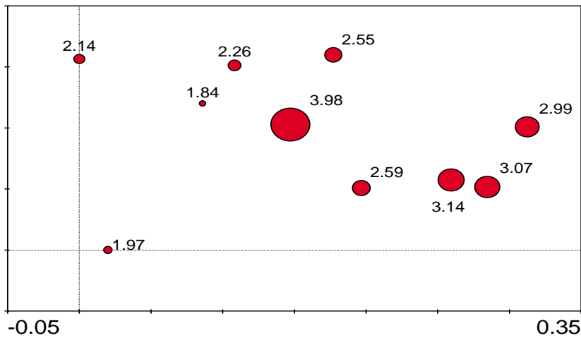
Fig. 3. Symbol attribute plot diagram Showing Pb concentration in C. sativa Site B.
