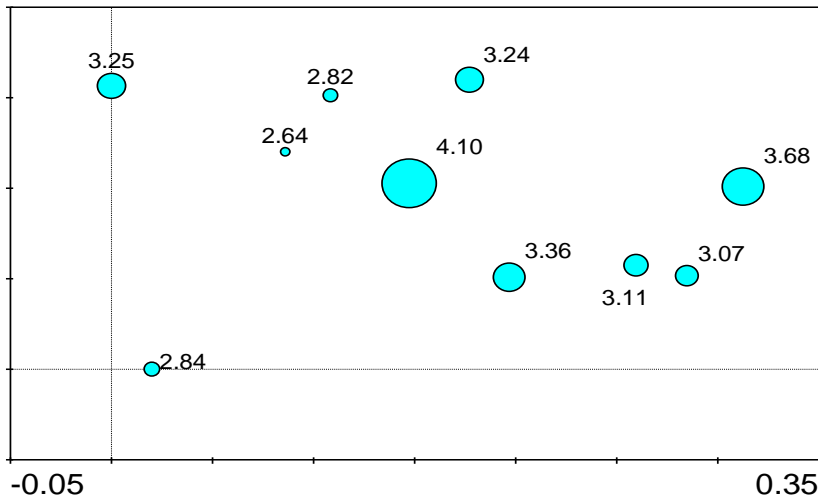
Fig. 2. Symbol attribute plot diagram showing Pb concentration in C. sativa Site A.
