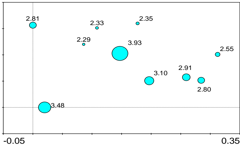
Fig. 4. Symbol attribute plot diagram Showing Pb concentration in D. sissoo Site A.
