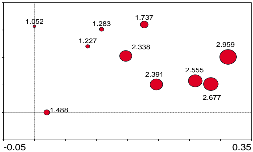
Fig. 5. Symbol attribute plot diagram Showing Pb concentration in D. sissoo Site B.
