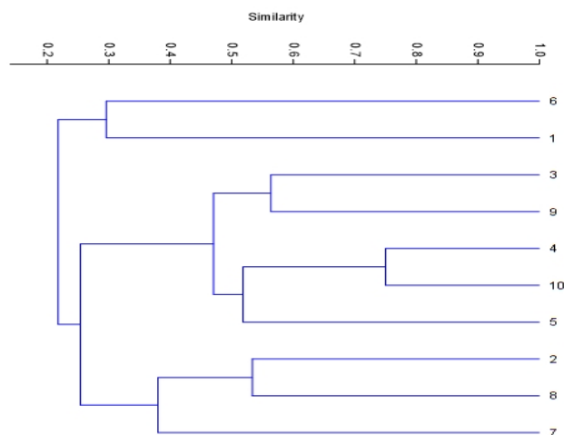
Fig. 15. The dendrogram of the connections between the study stations. 1: Juwaibdah 2: Hartha 3: Jabal Sanam 4: Khader Al-May 5: Um-Qaser 6: South Rumaila 7: Zariji 8: Qarmat Ali 9: North Rumaila 10: Jrishan
