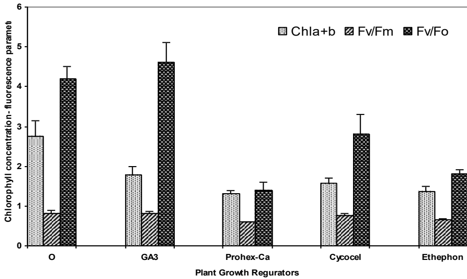
Fig. 1. Changes in chlorophyll a+b concentration ( \text{mg g}^{-1} \text{FW} ) and some chlorophyll fluorescence parameters ( n=5 ,) of Capsicum annuum L. cv 'Standar p.13/0211003-01-Agris' fully expanded leaves, as a function of PGRs application. Vertical bars represent the standard error.
