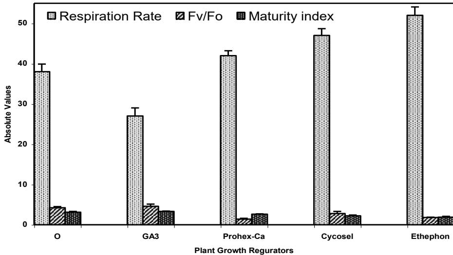
Fig. 2. \text{CO}_2 production ( \text{mgCO}_2 \text{ kg}^{-1} \text{h}^{-1} ) ( n=3 ), Fv/Fo ( n=5 ) and maturity index (Soluble Solids/Titratable Acidity) ( n=3 ) of Capsicum annuum L. cv 'Standar p.13/0211003-01-Agris' as affected by the application of PGRs. Vertical bars represent the standard error.
