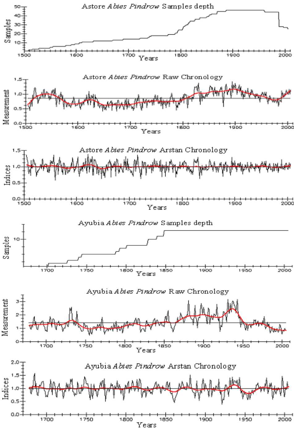
Fig. 1. Comparison of two individual chronologies of Abies pindrow . Outcome of standardization program ARSTAN.
