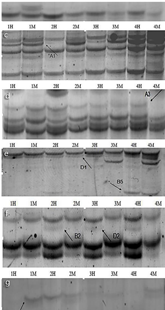
Fig. 1. Soybean leaf DNA methylation banding patterns Note: H: Eco R I+ Hpa II combination; M: Eco R I+ Msp I combination; 1: Long pin 09-85(control); 2: Long pin 09-85 (vaccination); 3: Yu nong 09-521 (control); 4: Yu nong 09-521 (vaccination)
