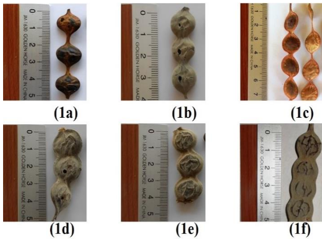
Fig. 1. Typical pods shape, color, texture, and constriction pattern of the subspecies nilotica (1a), tomentosa (1b), the new group (1c), and the subspecies adstringens (1d, 1e, and 1f).
