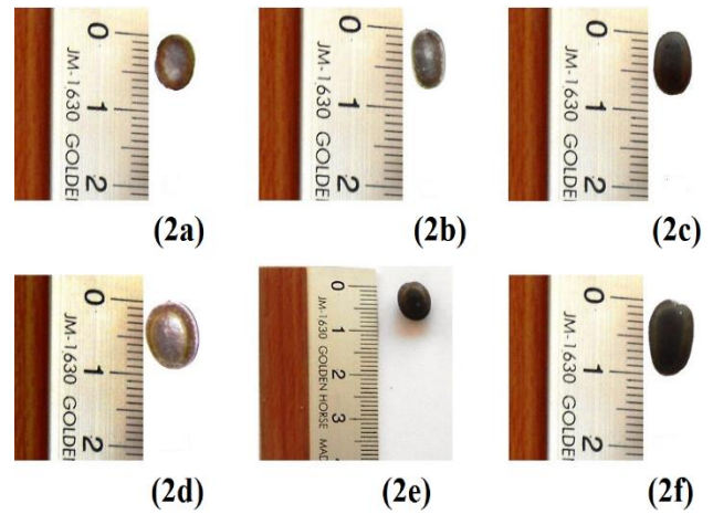
Fig. 2. Typical seed shape, colour, and texture of the subspecies nilotica (2a), tomentosa (2b), the new group (2c), and the subspecies adstringens (2d, 2e, and 2f).
