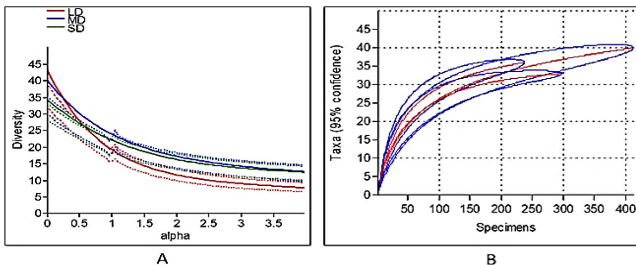
Fig. 2. (a) Comparative Rényi diversity profiles (b) species accumulation curves in the sampled forest sites in the Kupwara District of Kashmir region.
