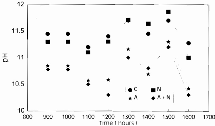
Fig.2.Kinetics of floodwater pH during day time in rice-Azolla culture (C = control, N = nitrogen avg. of T6 & T11, A = Azolla avg. of T2 & T3, A+N = T7).
