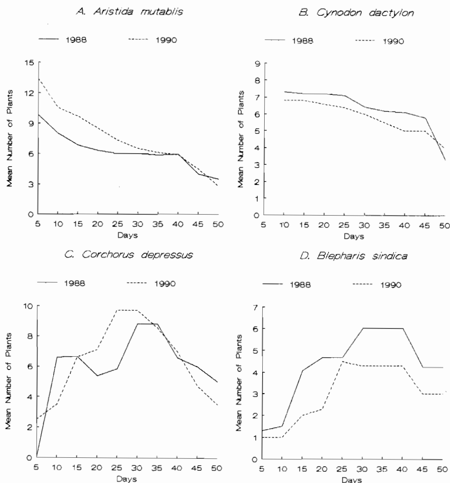
Fig. 3. Survivorship curve in 20 x 20 cm quadrats during 1988 and 1990 growing seasons. A, Aristida mutabilis ; B, Cynodon dactylon ; C, Corchorus depressus and D, Blepharis sindica .
