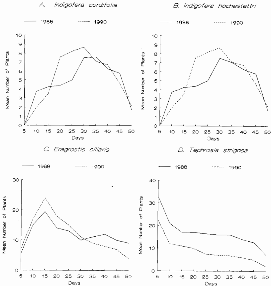
Fig. 2. Survivorship curve in 20 x 20 cm quadrats during 1988 and 1990 growing seasons. A, Indigofera cordifolia ; B, Indigofera hochestetri ; C, Eragrostis ciliaris and D, Tephrosia strigosa .
