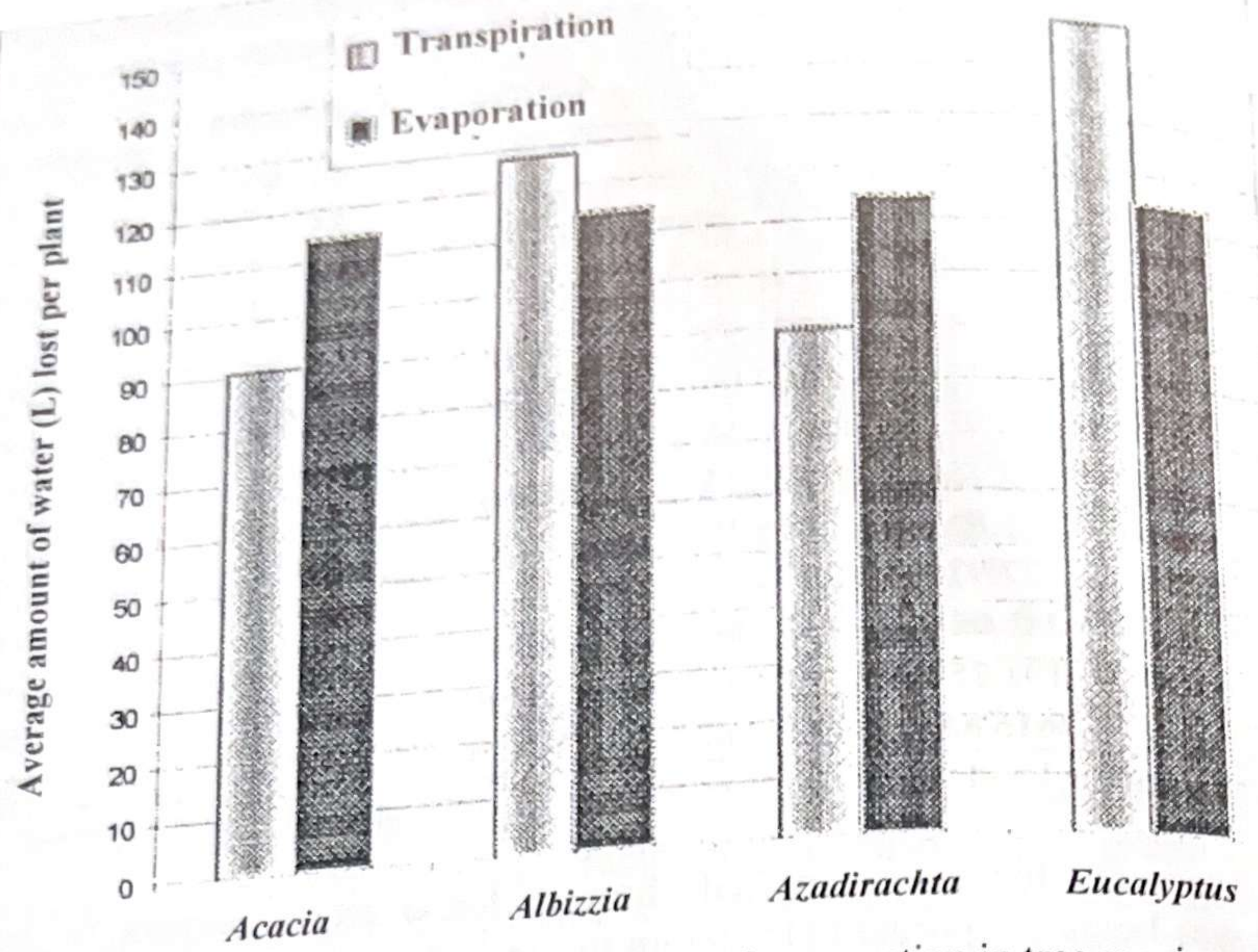
Fig. 1. Comparative transpiration and related evaporation in tree species.
