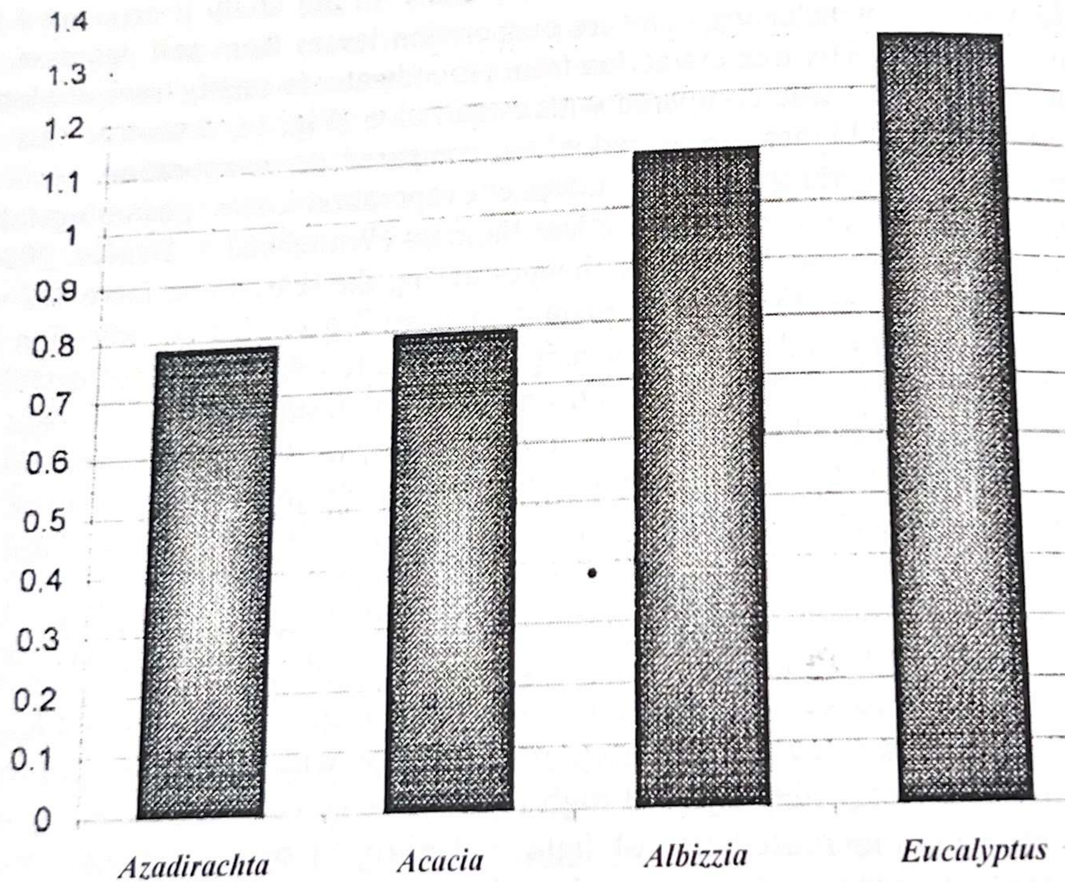
Fig. 2. Transpiration: Evaporation (T:E) Index of different tree species.
