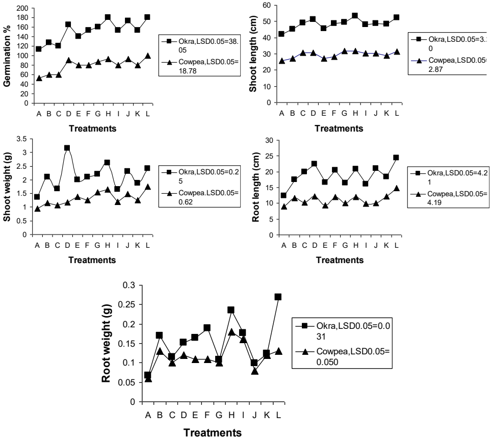
Fig. 1. Effect of plant extract alone and in combination with microbial antagonists on growth parameters of cowpea and okra. A= Control, B = Soil drenching with D. alba , C = seed treated with R. meliloti , D = B+C, E = seed treatment with T. harzianum , F = B+E, G = seed treatment with P. variotii , H= G+B, I = soil drenching with C. dactylon , J = I+C, K = I+E, L = I+G
