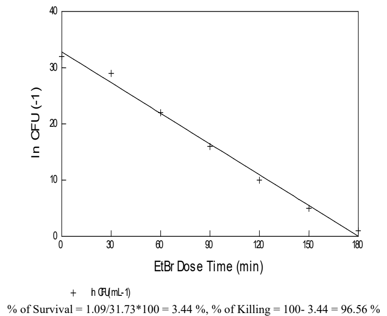
Fig. 3. Dose plot of ethidium bromide used for formulating the kill curve.
