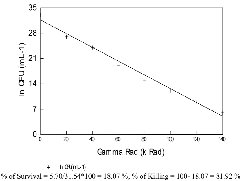
Fig. 2. Dose plot of gamma radiation to formulate the kill curve.
