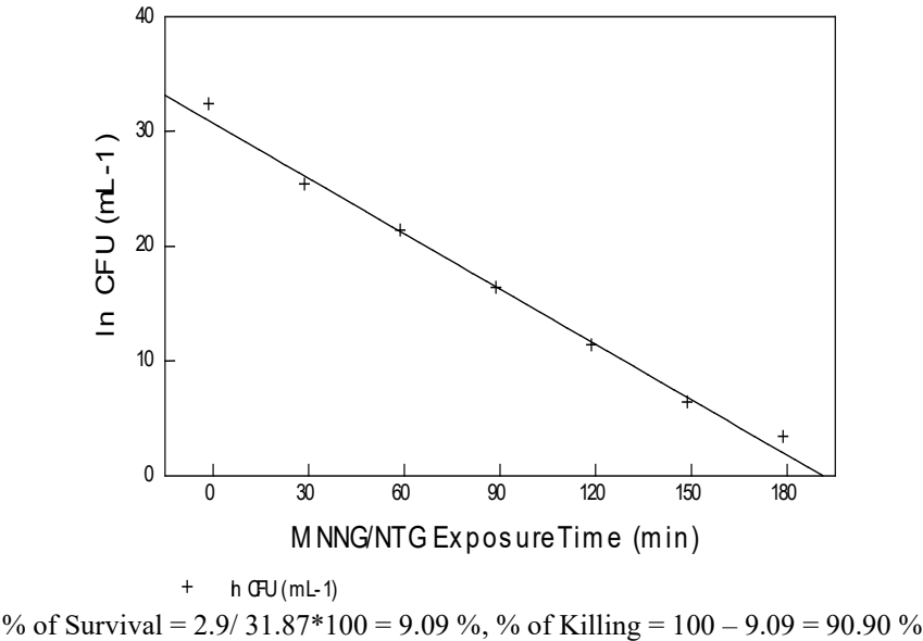
Fig. 5. Dose plot of MNNG/NTG to formulate the kill curve.
