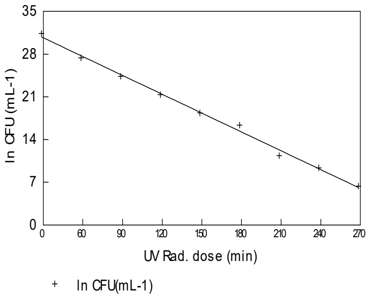
Fig. 1. Dose plot of UV to formulate the kill curve.
