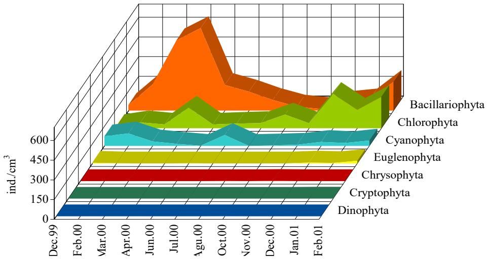
Fig. 2c. The seasonal changes of density of phytoplankton groups of Lake Sapanca at station 3.
