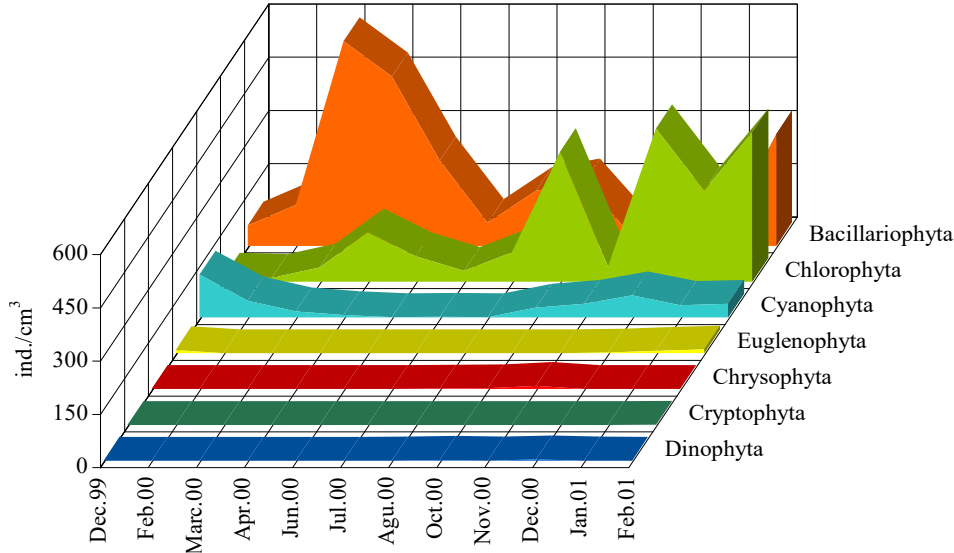
Fig. 2b. The seasonal changes of density of phytoplankton groups of Lake Sapanca at station 2.
