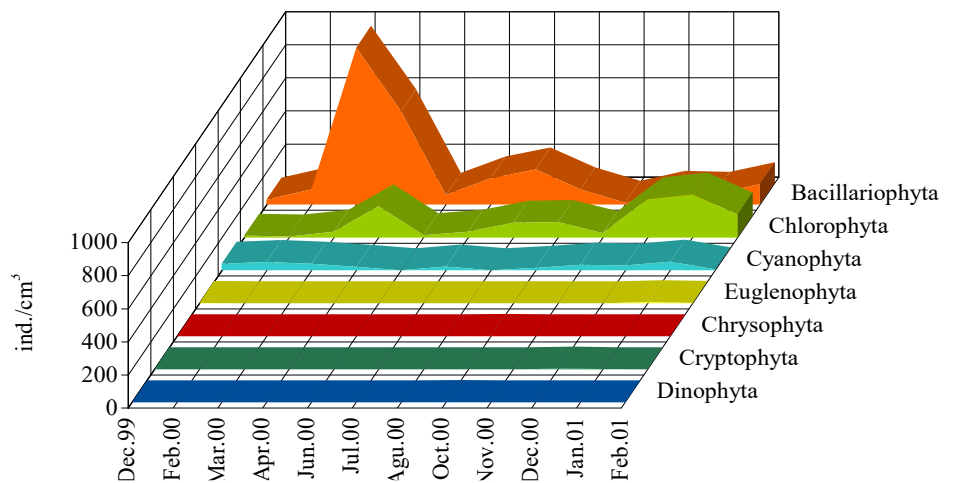
Fig. 2d. The seasonal changes of density of phytoplankton groups of Lake Sapanca at station 4.
