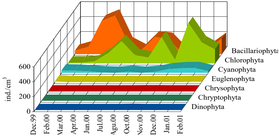
Fig. 2a. The seasonal changes of density of phytoplankton groups of Lake Sapanca at station 1.
