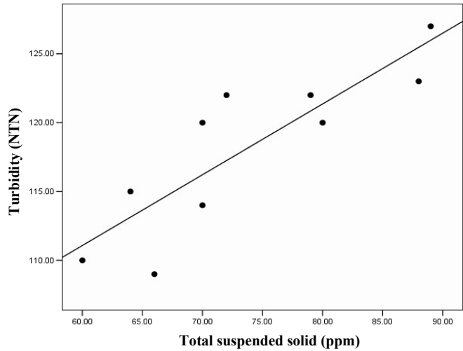
Fig. 11. Regression line between turbidity and total suspended solids.
