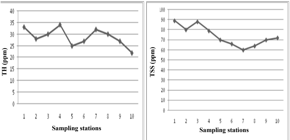
Fig. 3. Average Total Suspended Solids (TSS) & Mean Total Hardness (TH) in ppm calculated at selected sampling sites of the River Chenab.
