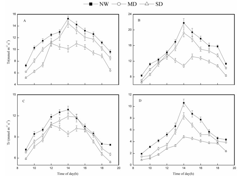
Fig. 5. Diurnal patterns of Tr under different watering regimes in different growth stages. a, b, c, d refers to five-leaf stage- June 17; jointing stage- July 11; flowering stage- August 19; soft dough stage- September 1.
