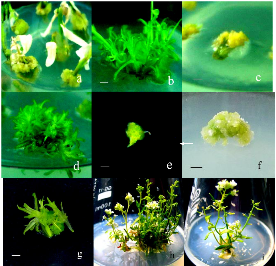
Fig. 1. Plantlet regeneration and flower inducing of Thellungiella salsuginea . (a) After 3 weeks' culture stem callus formed (bar 5 mm). (b) Shoots regenerated from stem callus after 3 weeks' culture (bar 2.5 mm). (c) Yellow leaf callus formed after 3 weeks' culture (bar 2.5 mm). (d) Shoots regenerated from leaf callus (bar 2.5 mm). (e) Green callus formed from anthers. The arrow shows blasted filament (bar 1 mm). (f) Three-time subcultured anther callus (bar 5 mm). (g) Shoots regenerated from anther callus (bar 5 mm). (h) Shoots regenerated from anther callus (bar 5 mm). (i) Shoots fruited 4 weeks later after be transplanted on MS medium (bar 5 mm).
