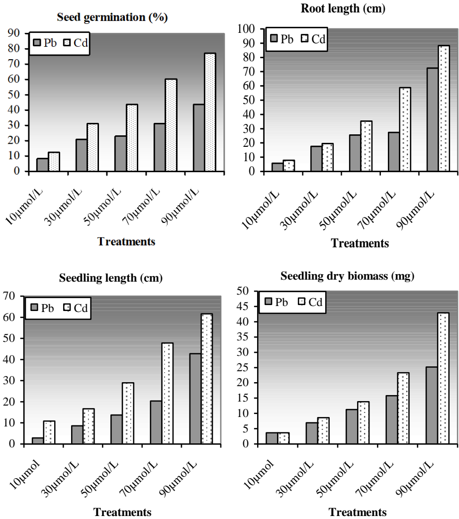
Fig. 1. Percentage decrease in seed germination, seedling length, root length and seedling dry biomass of Albizia lebbek at different concentrations of lead and cadmium as compared to control.
