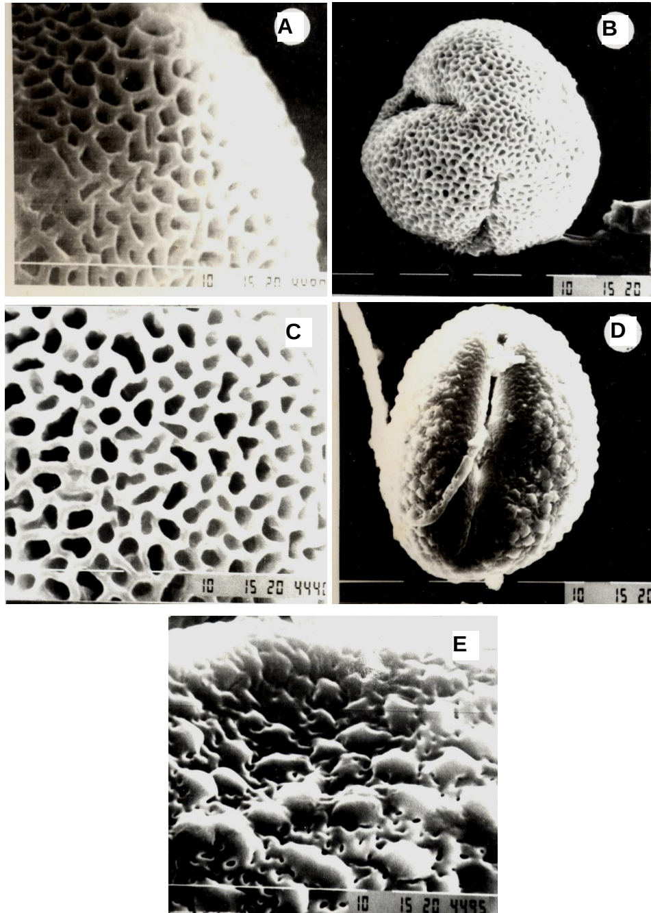
Fig. 2. Scanning Electron micrographs of pollen grains. Ctenolepis cerasiformis : A, Polar view; Momordica charantia : B, Polar view, C, Exine pattern. Solena amplexicaulis : D, Equatorial view; E, Exine pattern Scale bar = 10 \mu m.
