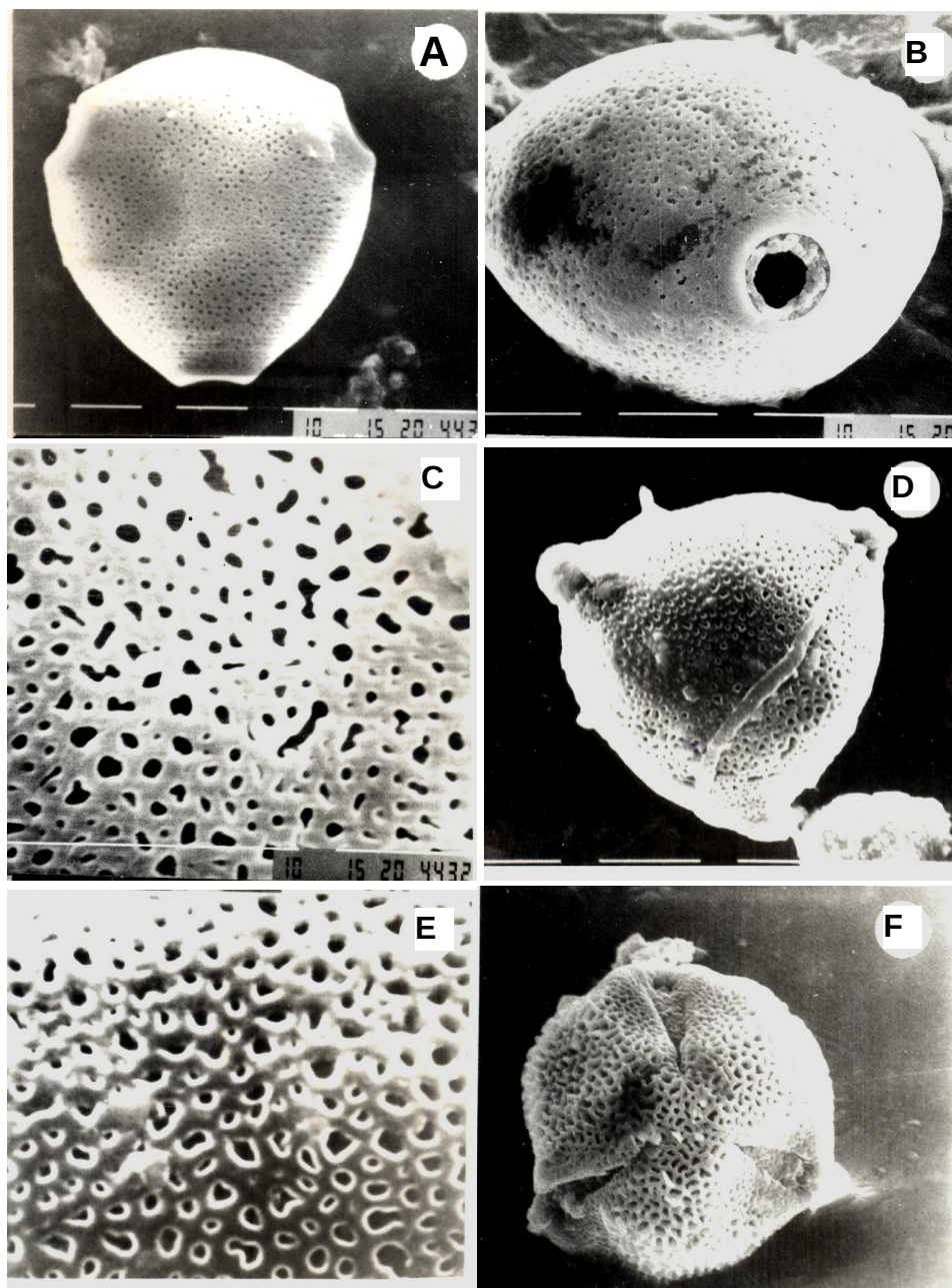
Fig. 1. Scanning Electron micrographs of pollen grains.: A, Cucumis melo ssp. agrestis Polar view, B, Equatorial view; C, Exine pattern. Mukia maderspatana : D, Polar view; E, Exine pattern. Ctenolepis cerasiformis F, Polar view. Scale bar = 10 \mu m.
