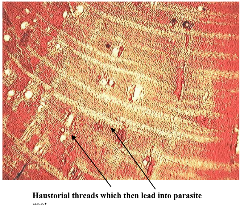
Fig. 6. Further ramification of haustorial threads in mid-central xylem of the host root.
