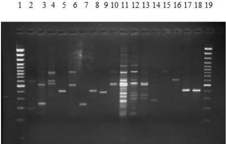
Fig. 1. RAPD profiles of genomic DNA of Alfred, Paars and control samples of Rhododendron . Lane 1 and 19. Molecular size marker (100 bp molecular size ladder), Lane 2-Lane 18: KA1, KA2, KA3, A2, A3, A4, A5, A6, A9, KB, B2, B3, B4, B5, B6, B7, B9.
