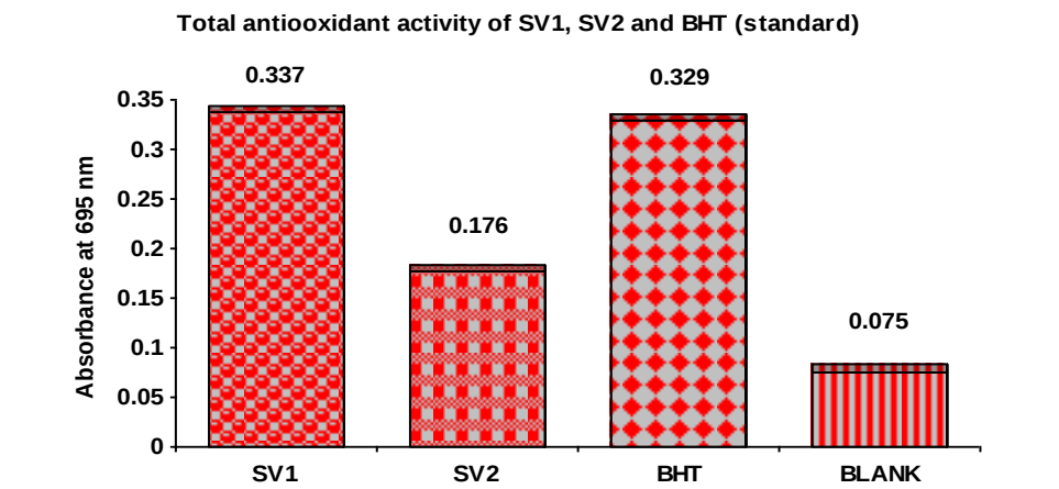
Fig. 2. Total antioxidant capacity assay.
