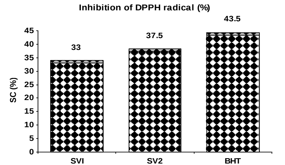
Fig. 1. DPPH free radical scavenging activity of Extracts and a standard antioxidant BHT.
