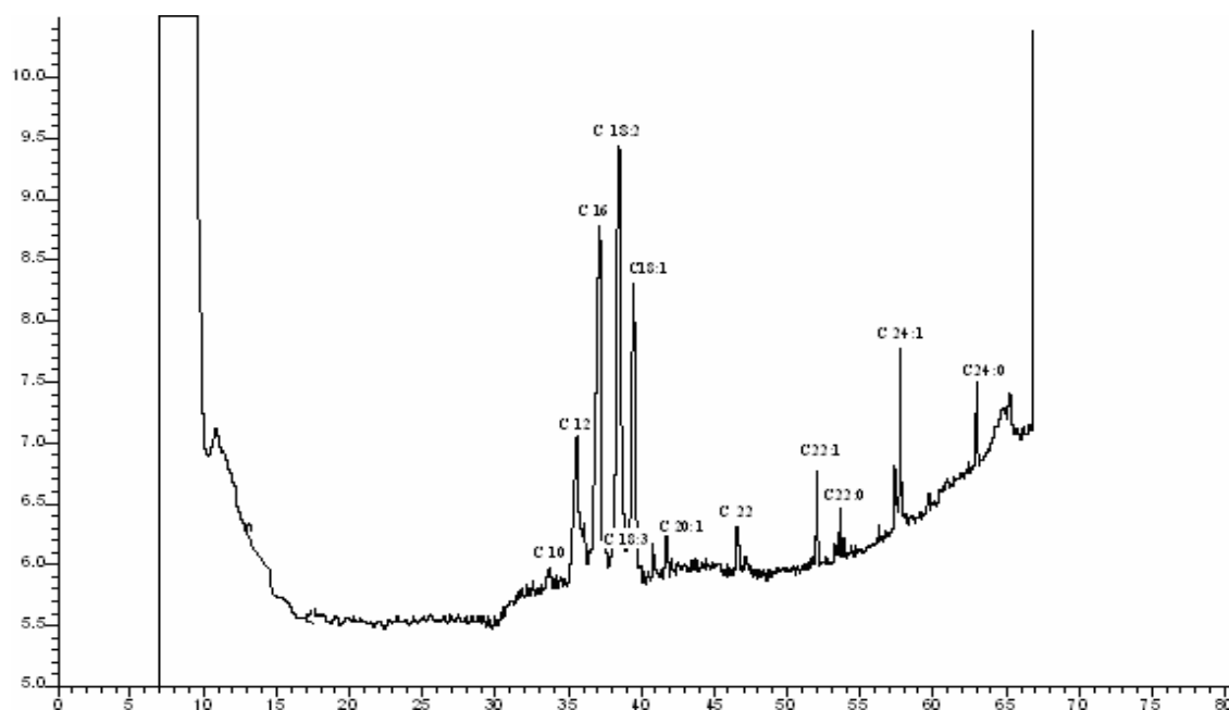
Fig. 1. GC Chromatogram obtained by the injection of 5 \mu\text{L} of fatty acid (methyl esters) from Eruca seeds.
