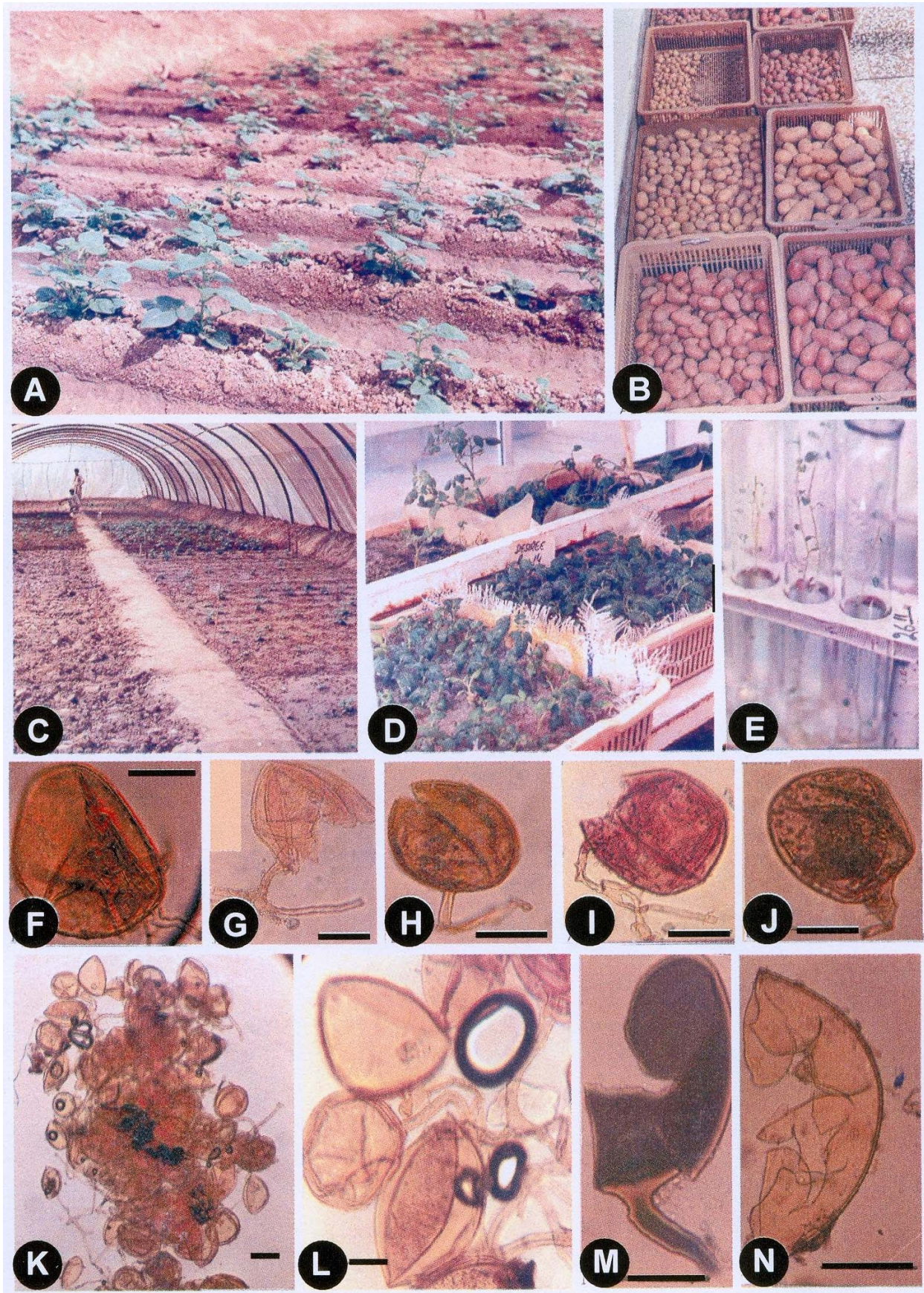
Fig. 4. A-E: Tissue culture raised potato plantlets in growth tunnels, test trays and tubes in Sahiwal area of Pakistan. F: Glomus albidum . G & H: Glomus claroideum ; I: Glomus microcarpum ; J: Glomus multicaule ; K & L: Glomus mosseae ; M: Glomus monosporum ; N: Glomus sp. (bar = 30 μm).
