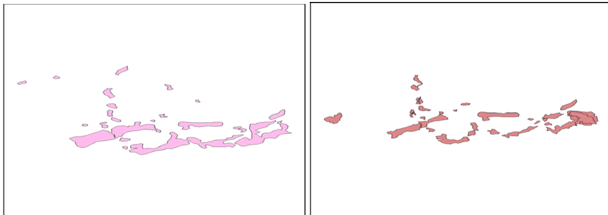
Fig. 1. Forest cover in Chakwal District 2005-06.
