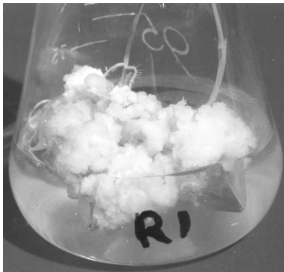
Fig. 1. Callus induction on rice caryopsis cultured on MS medium containing 1.0 mg/l 2,4-D, 0.5 mg/l Kn and 50 mg/l tryptophan.
