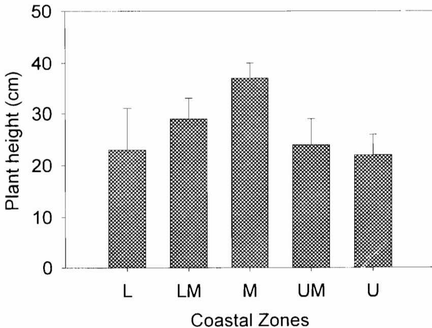
Fig.5. Height of Arthrocnemum macrostachyum plants collected from various coastal zones.
